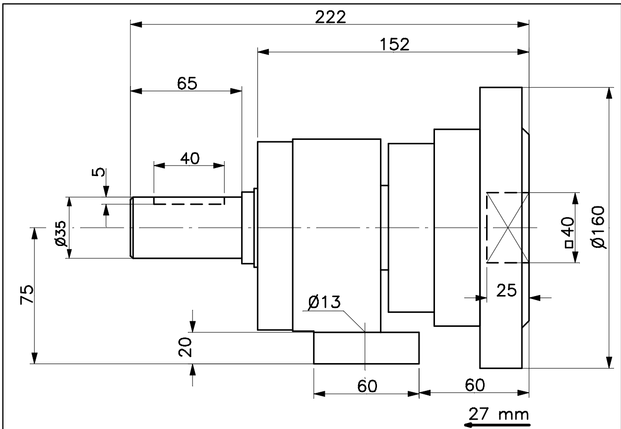
Pillow-Block Version
